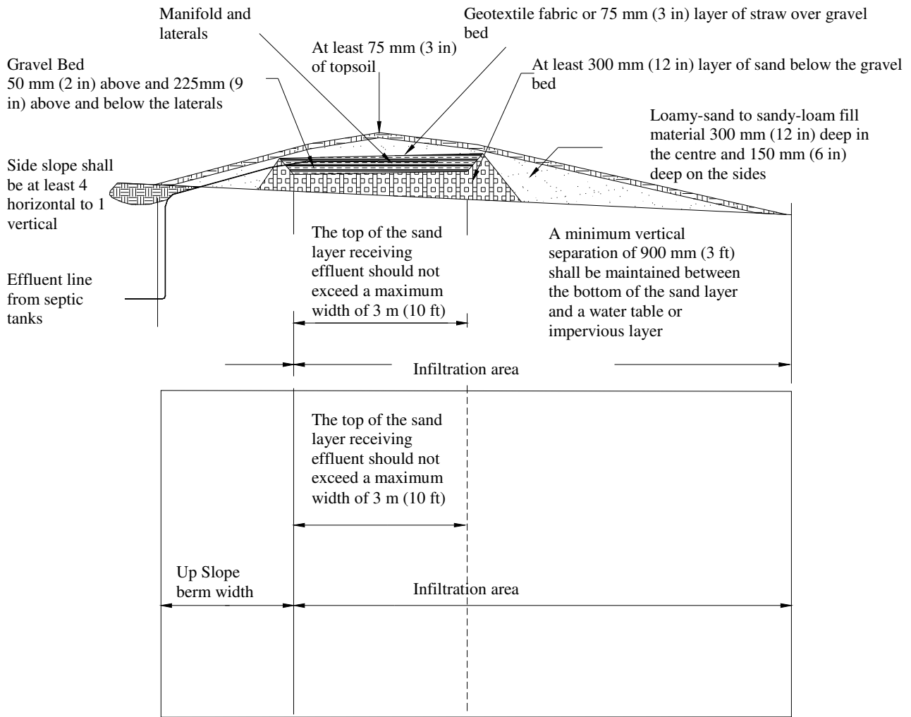
Figure 9.7 – Mound on slope
