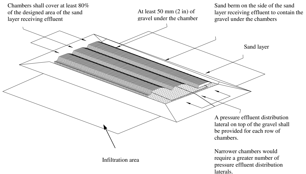
Figure 9.5 – Chamber Mound
