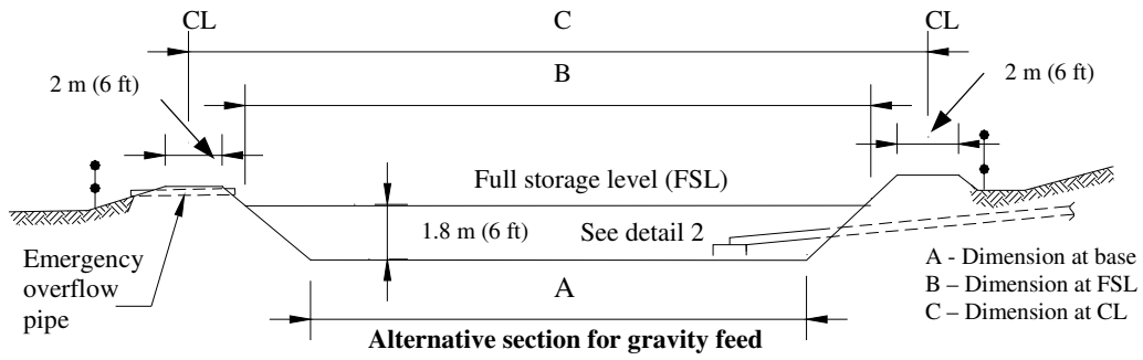
Figure 11.2 – Sewage Lagoon Sizing
