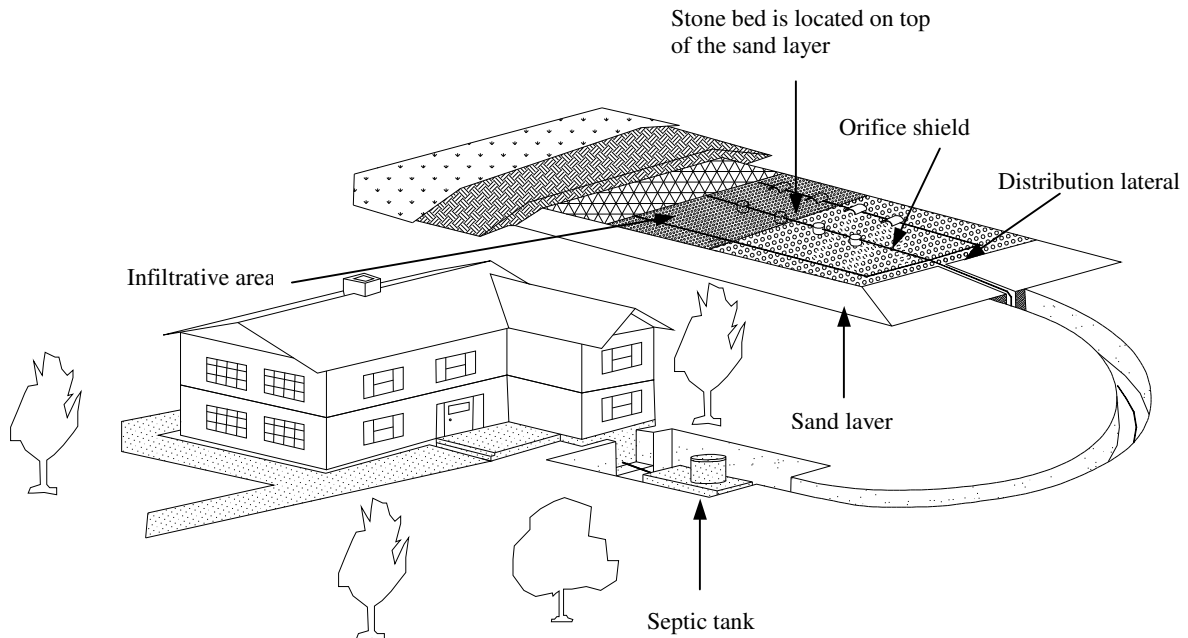
Figure 9.4 Type II Mound
